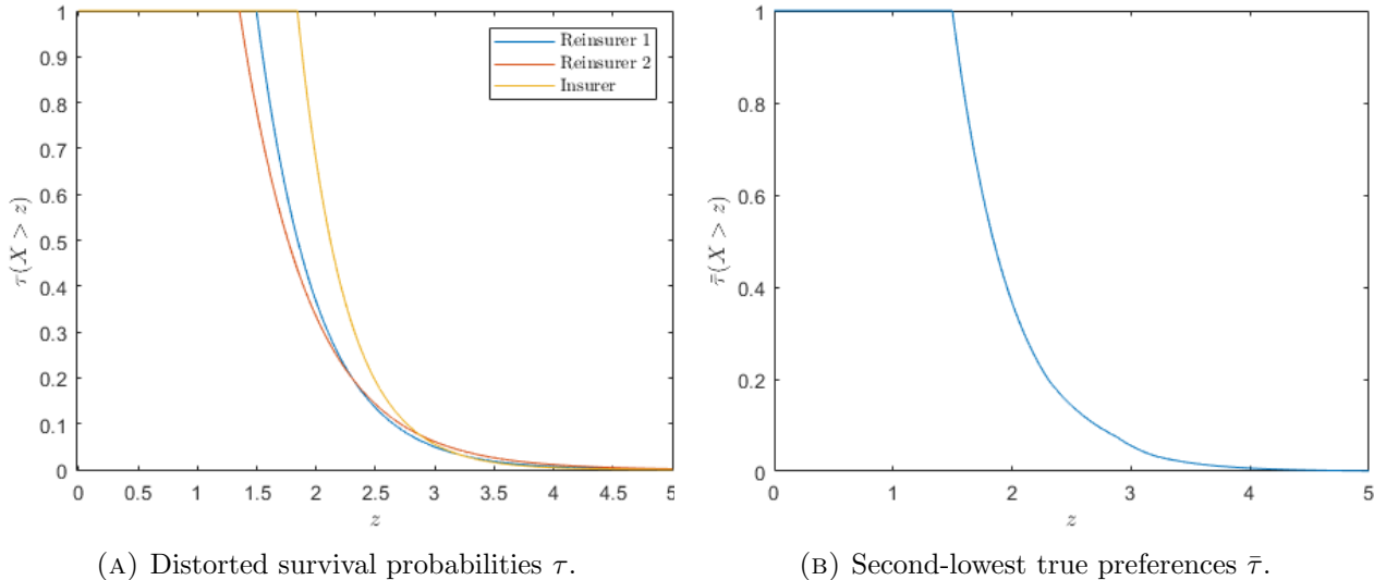
FIGURE 1. Survival functions of true preferences.
