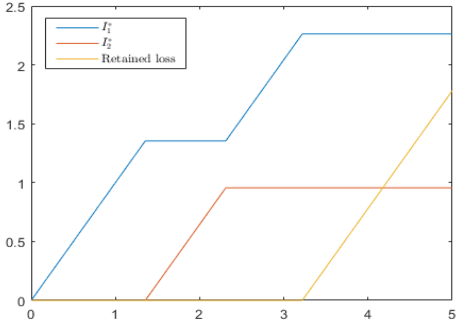
FIGURE 2. Optimal indemnity structure \vec{I}^* .
