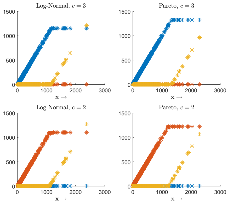
Figure 1: Pareto optimal risk allocations (\mathbf{y}^*, \mathbf{z}^*, \mathbf{t}^*) that solve (4.8) and are respectively displayed in blue, red and yellow. The left and right panels show the Log-Normal and Pareto sample, respectively; the top and lower panels correspond to the c = 3 and c = 2 case, respectively.
