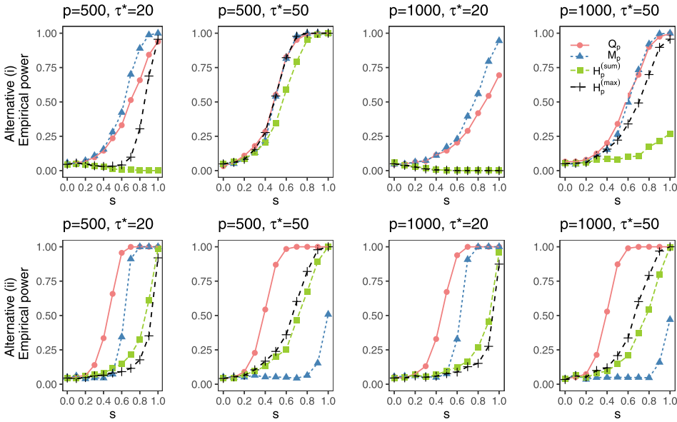
FIG. 3. Comparison of size-corrected empirical power under the alternative hypotheses (i) and (ii).
